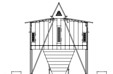
Back Elevation
